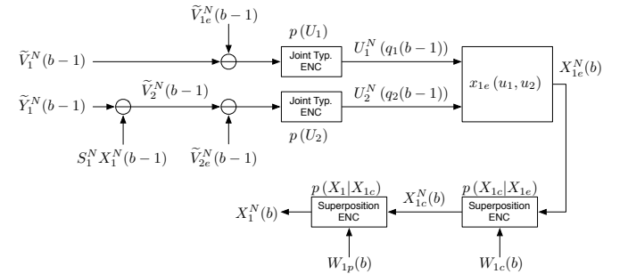
Fig. 2. Block Diagram of Encoder at Tx1
